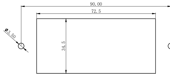
PANEL CUT-OUT
